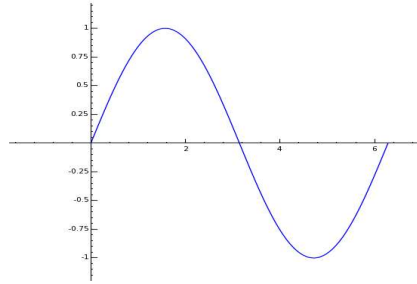
Figure 1: Solution to IVP x'' + x = 0 , x(0) = 0 , x'(0) = 1 .
