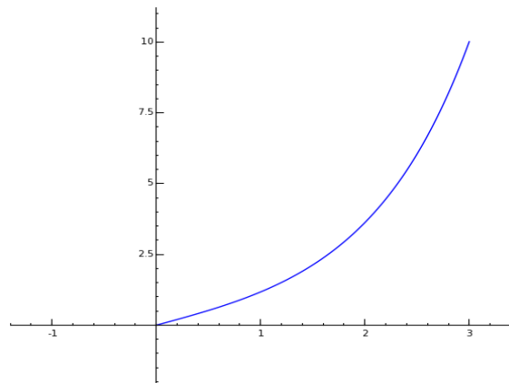
Figure 3: Solution to IVP x'' - x = 0 , x(0) = 0 , x'(0) = 1 .
