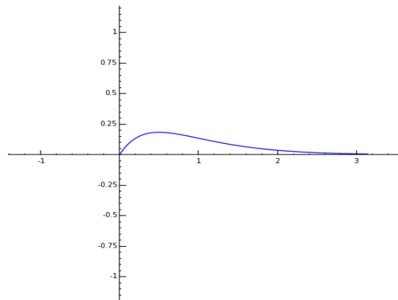
Figure 2: Solution to IVP x'' + 4x' + 4x = 0 , x(0) = 0 , x'(0) = 1 .
